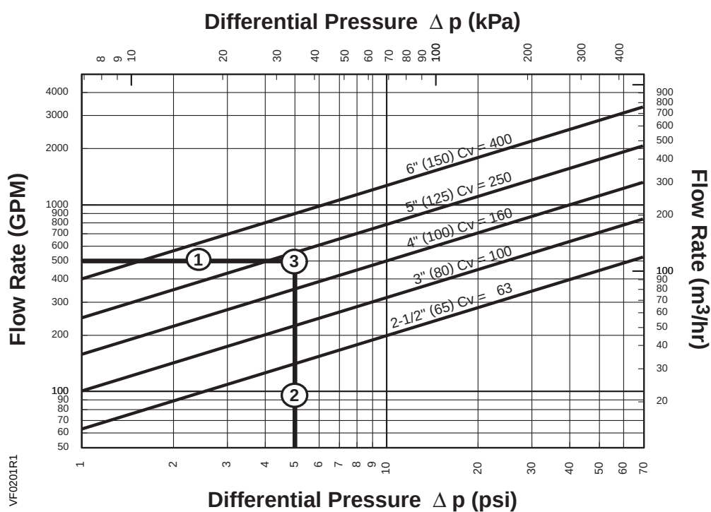
Figure 2. Water Capacity Graph.
