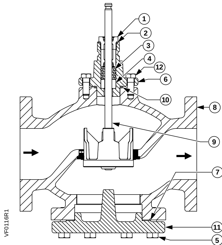
Figure 5. Two-Way Normally Closed.
