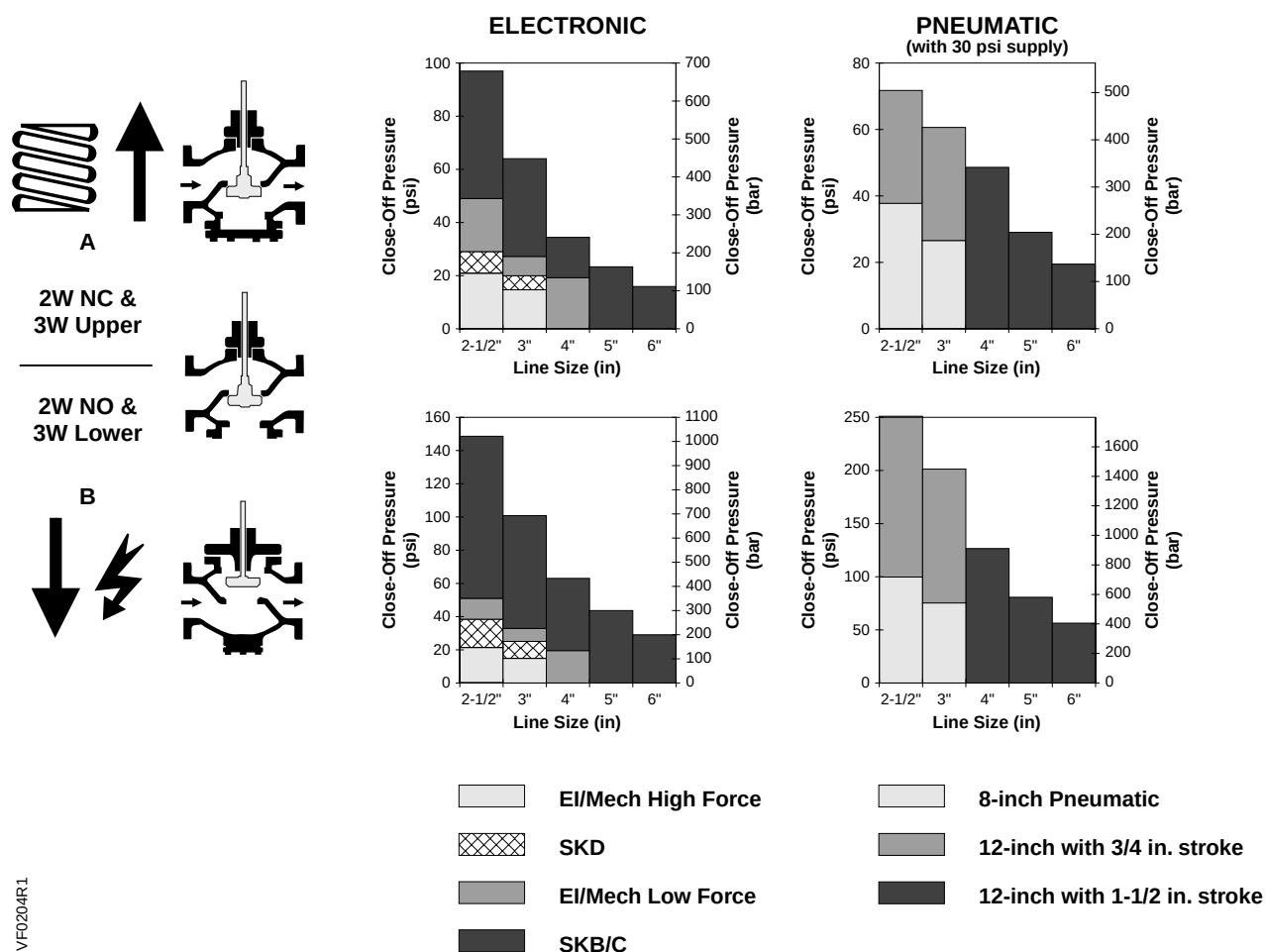
Figure 3. Close-off Pressures.
